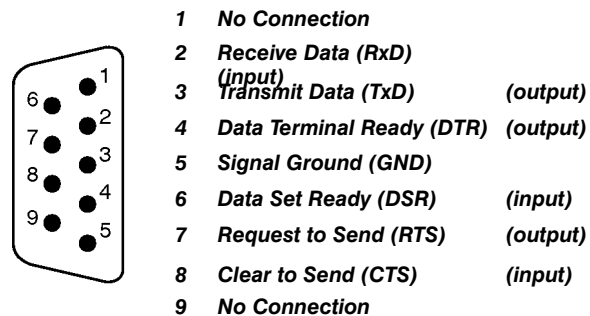
Figure 1-10: Pin Assignments of the RS-232 Connector
